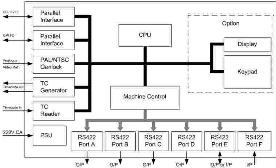
Figure 1: RM-6 block diagramme
